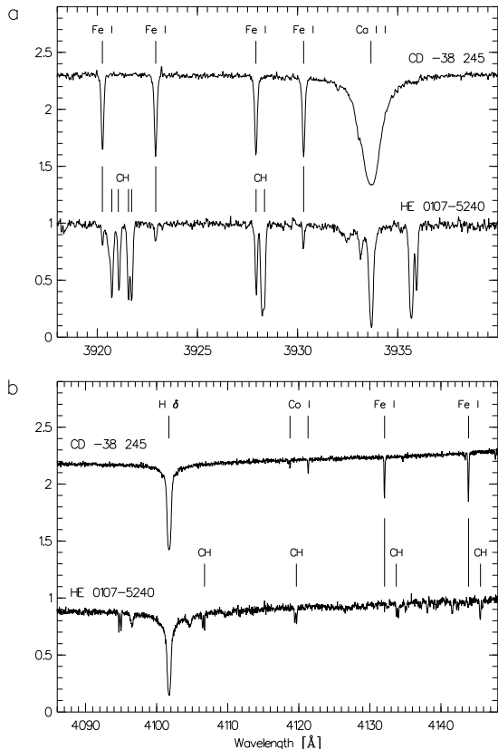
Figure 1: A portion of the spectrum of HE 0107–5240, shown compared to the spectrum of CD -38^{\circ} 245, the previously most iron-poor giant star known. Both spectra were obtained with VLT-UT2, and the Ultraviolet-Visual Echelle Spectrograph (UVES). We note the strong molecular CH and C 2 lines and extremely weak lines of Fe I in the spectrum of HE 0107–5240. The spectra used in our analysis have a resolution of R = \lambda/\Delta\lambda = 40,000 , and a signal-to-noise ratio of more than 100 per pixel at \lambda > 400.0 nm. The covered wavelength ranges are 329.0–452.0 nm, 478.0–576.0 nm, and 583.0–681.0 nm.
